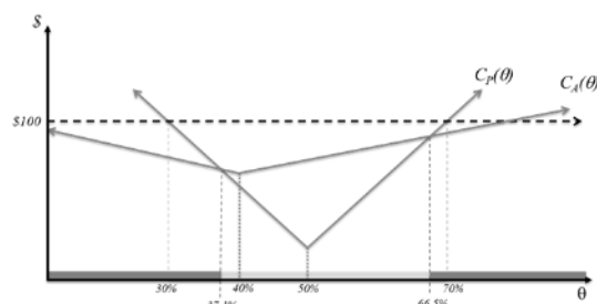
Figure 2c: Optimal COW Waives "All But" Specific Classes of Projects
