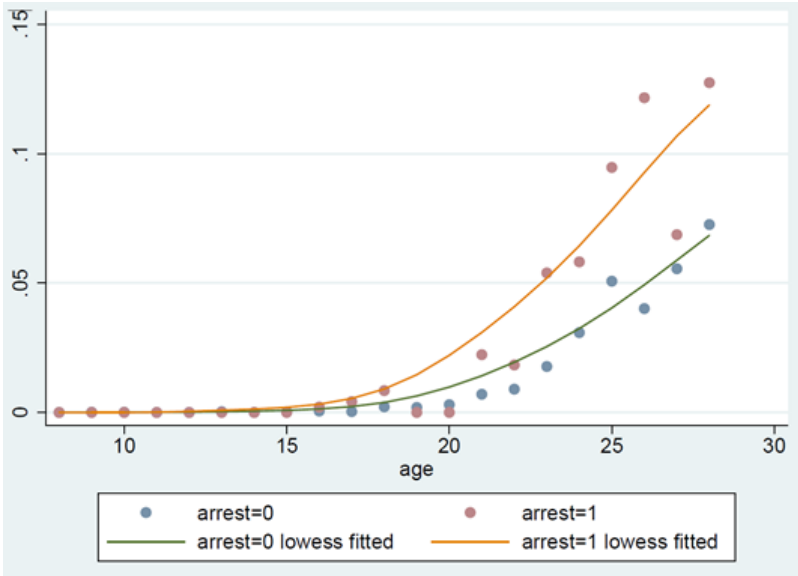
Figure 5: Hazard Regression
